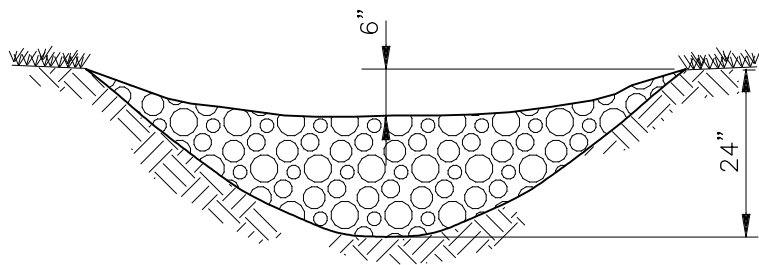
ROCK CHECK DAM
