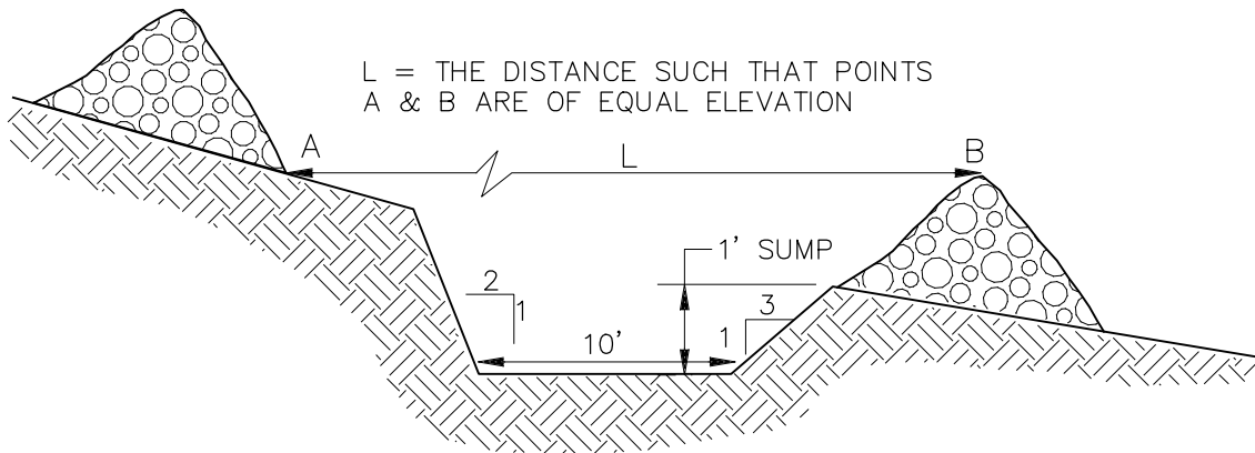
ROCK CHECK DAM CROSS-SECTION
