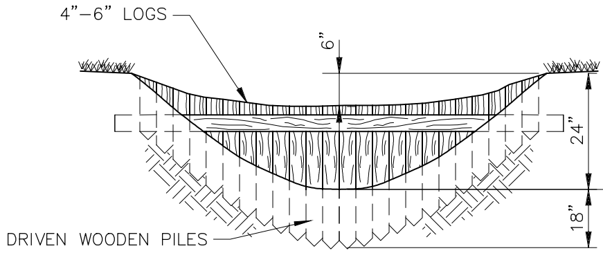
LOG CHECK DAM
