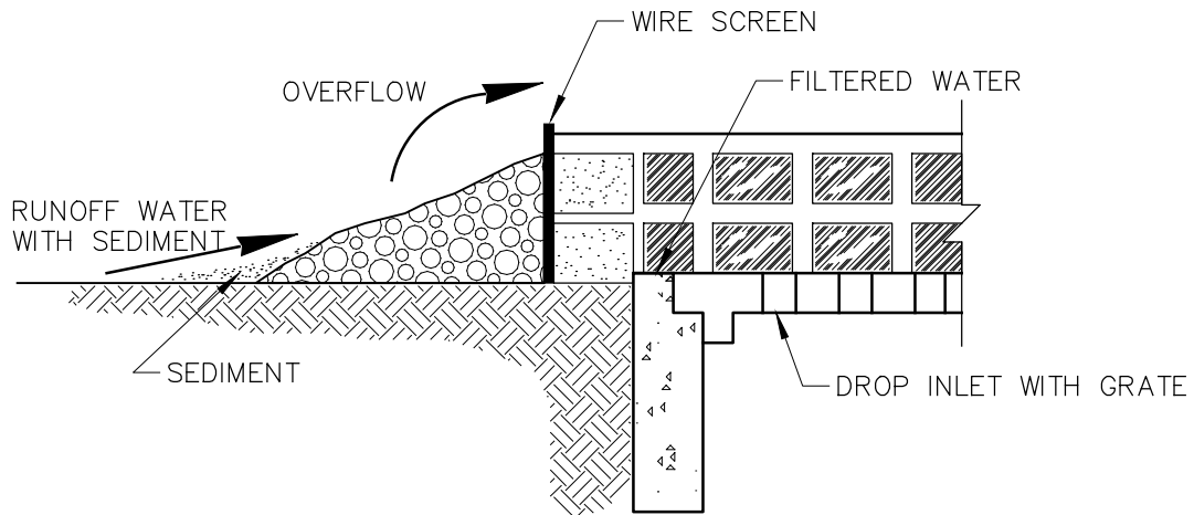
BLOCK AND GRAVEL FILTER AT DROP INLET
