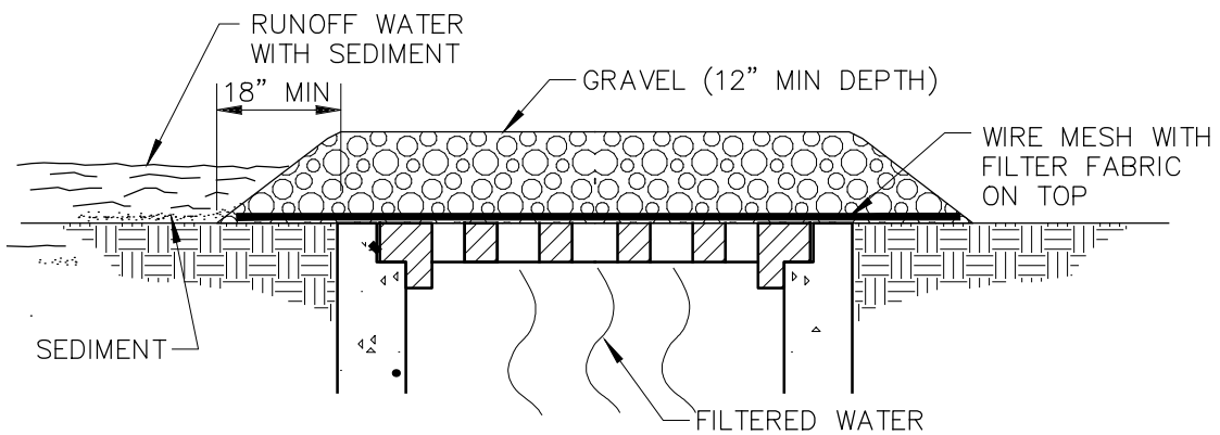
GRAVEL AND WIRE MESH FILTER
